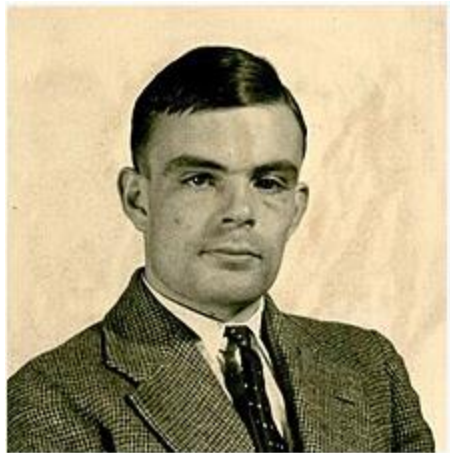
Turing in 1936
